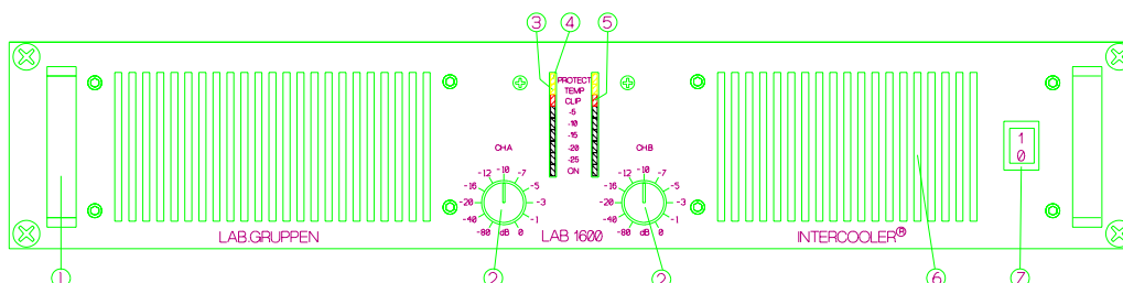
Figure 1. Front panel
